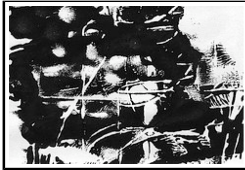
decomposition
