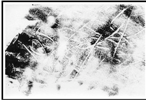
decomposition
