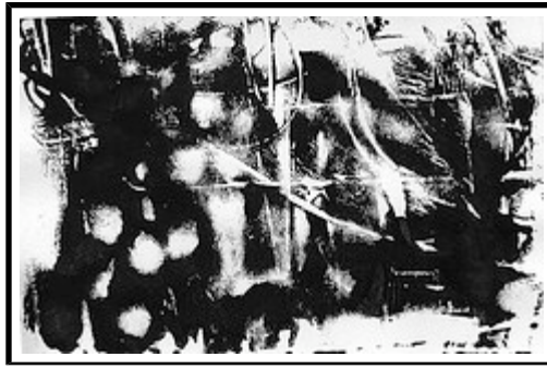
decomposition
